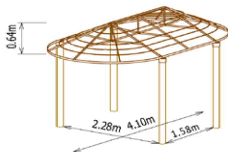
Savannalodge 2,80x4,50m :
