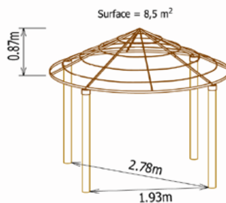
Savannalodge Ø 3,30m :
