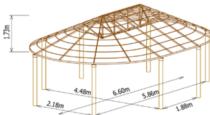
Savannalodge 5,00x7,00m :
