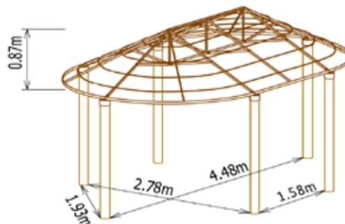
Savannalodge 3,30x5,00m :
