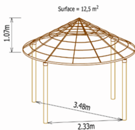
Savannalodge Ø 4,00m (4 poteaux) :
