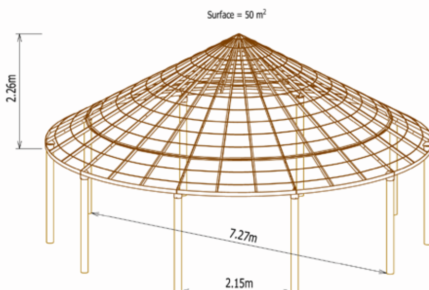
Savannalodge Ø 8,00m :
