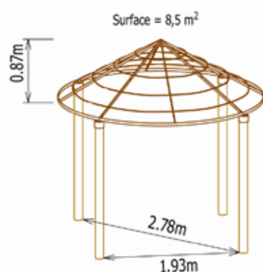
Savannalodge Ø 3,30m :
