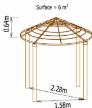
Savannalodge Ø 2,80m :
