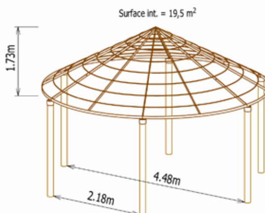
Savannalodge Ø 5,00m :
