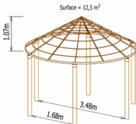
Savannalodge Ø 4,00m (6 poteaux) :
